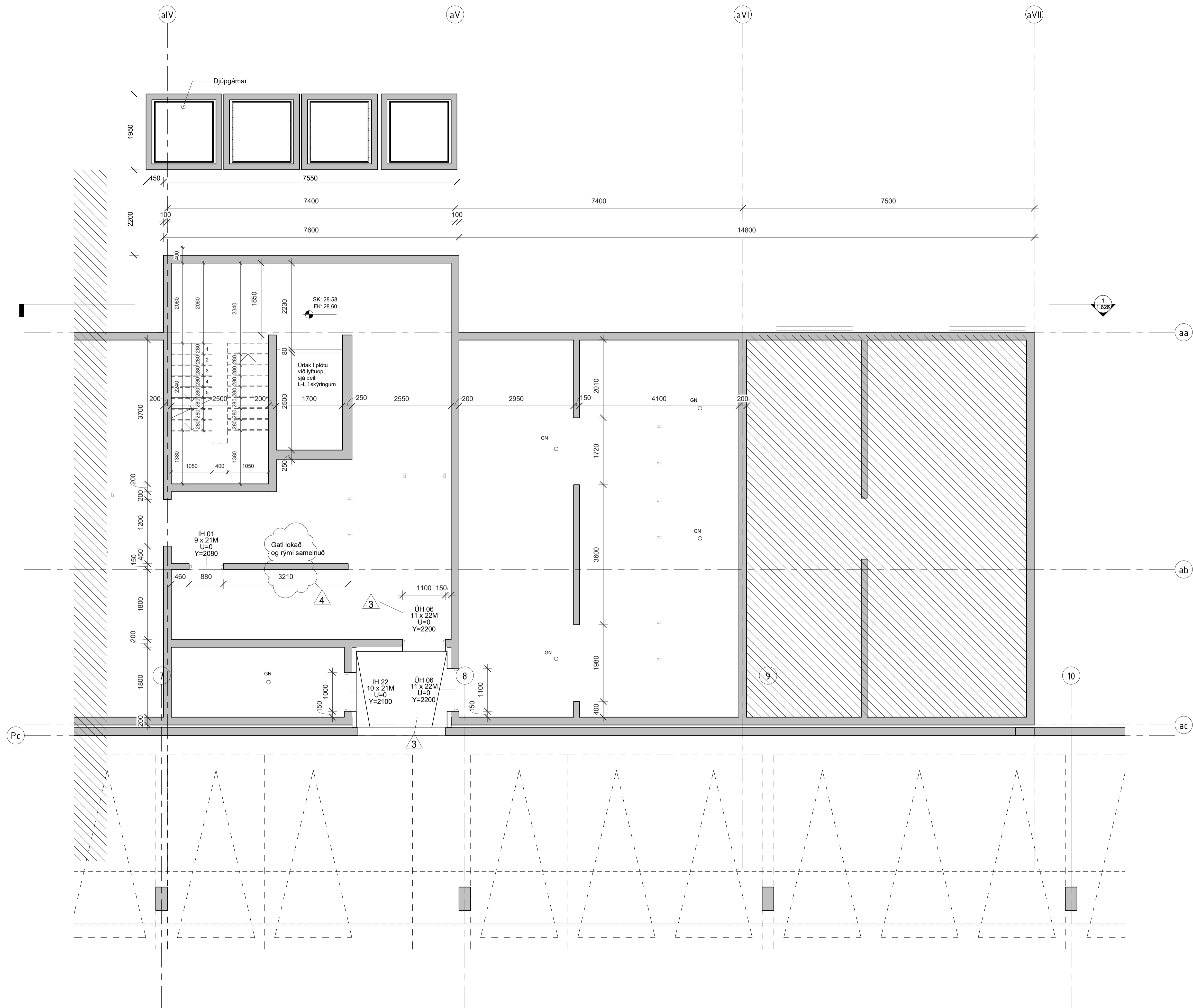
Kjallari-Steypa - sll 1 : 50
